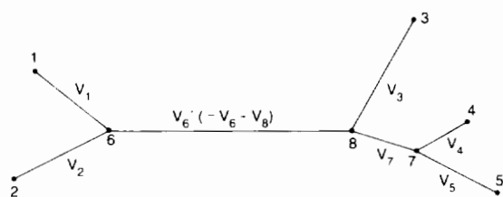
Fig. 3. The unrooted tree whose likelihood is equivalent to those in Fig 1 and 2
