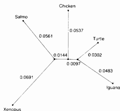
Fig. 4. The maximum likelihood estimate of the phylogeny for 5S RNA sequences from five vertebrate species
